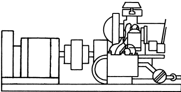
3 AE.N...-RG with flexible coupling and internal combustion engine
