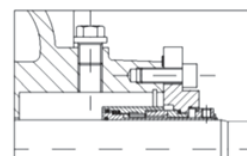
Figure 8: Cartridge type Mechanical Seal
