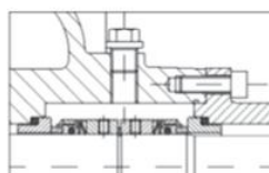
Figure 7: Double Mechanical Seal - with Flushing
