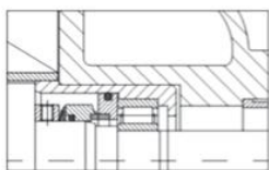
Figure 5: Internal Mechanical Seal
