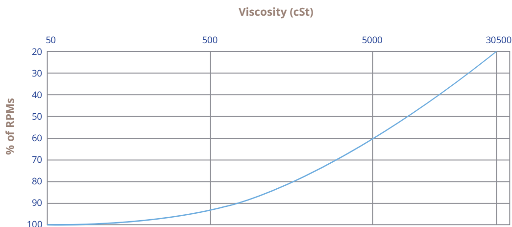
Percentage of RPMs on fluid Viscosity (cSt)
