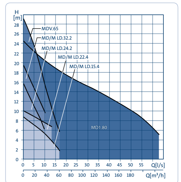
Pump performance
