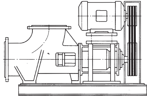
Propeller pump installed horizontally on base plate, motor aligned above bearing bracket, drive via V-belt.
