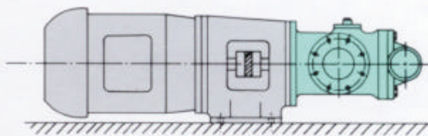
HORIZONTAL FACE MOUNTED UCF PUMP/MOTOR ASSEMBLY
