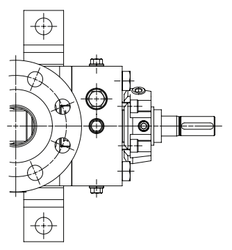
BASIC CARTRIDGE SEAL (13.5) WITH DEVIATIONS TO API 682
